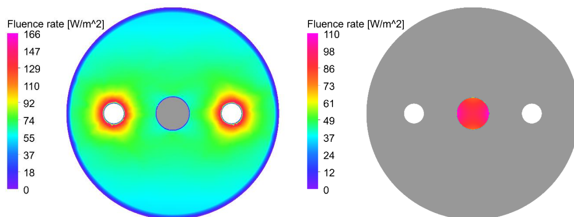
Fig. 5. Simulated fluence rate distribution contour at the middle cross-section of the photoreactor
