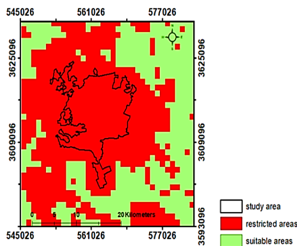
Fig. 1. Final suitability map from the Boolean overlay method
