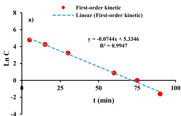
Fig. 8. Fitting the first-order (a) and second order (b) kinetic models to the decolorization data in the ozone-Electro-Fenton hybrid process
