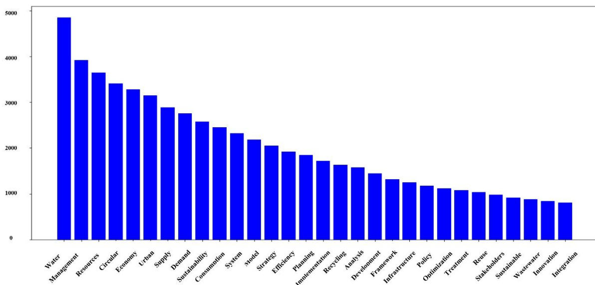
Fig. 4. The 30 most frequent keywords and their occurrences
