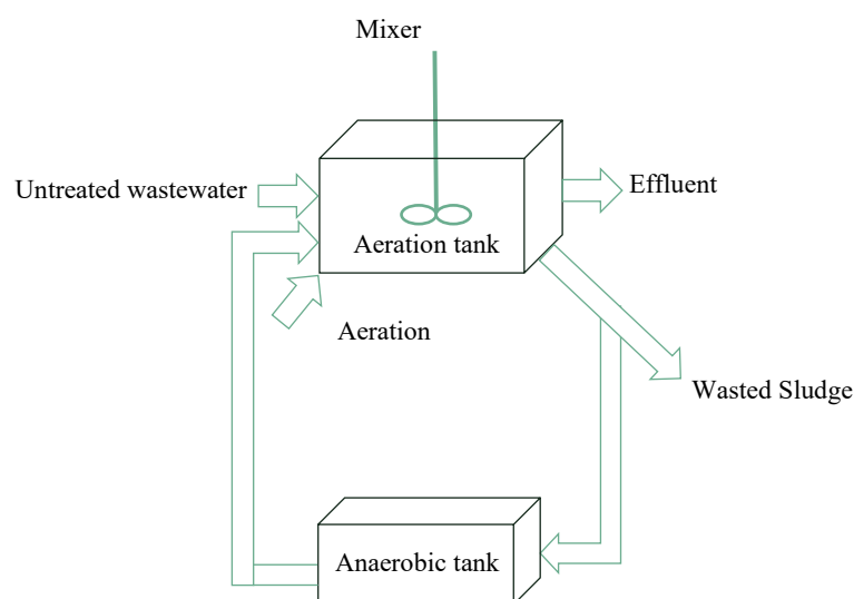
Fig. 3. The scchmeatic of the developed laboratory pilot
