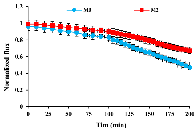
Fig. 6. Organic deposition of M0 and M2 membranes
