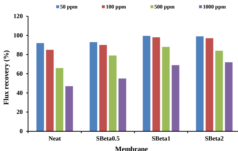
Fig. 9. Evaluating membrane flux recovery for the nanocomposite membrane across various feed concentrations
