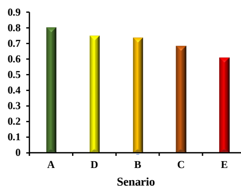
Fig. 2. Ranking of scenarios based on GFDM results
