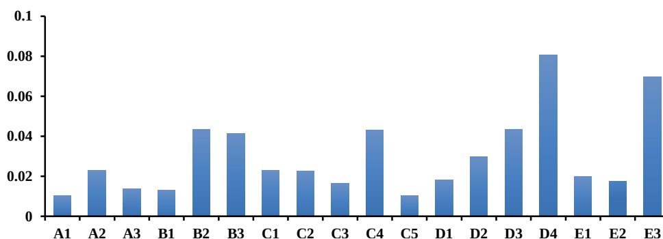
Fig. 3. Final weights of the sub-criteria
