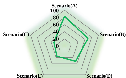
Fig. 6. Scenario scores based on sensitivity analysis of the environmental criterion
