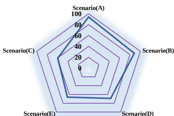
Fig. 7. Scenario scores based on sensitivity analysis of the technical criterion
