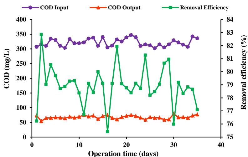
Fig. 3. Variations of COD in the MBR influent (raw wastewater) and MBR effluent (treated wastewater), and its removal efficiency during the operation period
