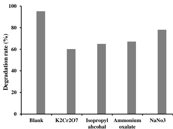
Fig. 13. The effect of different radical absorbers on photocatalytic degradation of DR16
