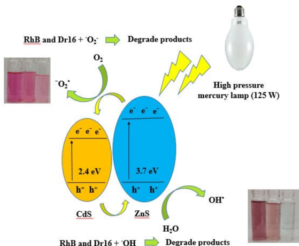
Fig. 12. Photocatalytic decomposition of organic dyes in the presence of Fe_3O_4@BNPs@ZnS-CdS
