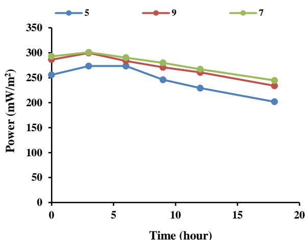
Fig. 10. Diagram of power density-time at different pH
