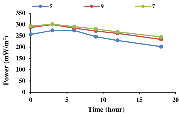
Fig. 4. Diagram of power density-time at different pH
