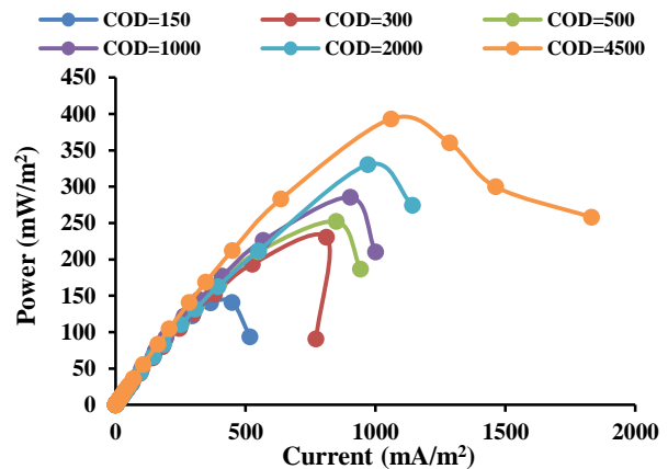
Fig. 8. Diagram of different COD concentration
