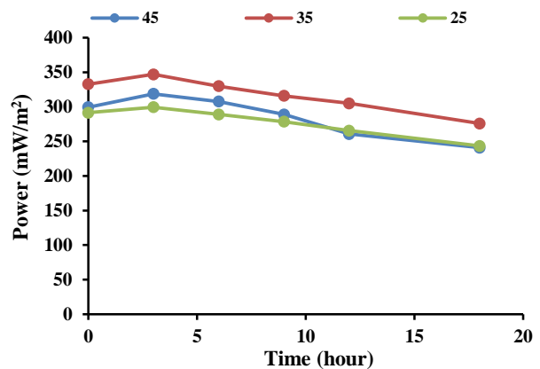
Fig. 9. Diagram of power density-time at different temperatures
