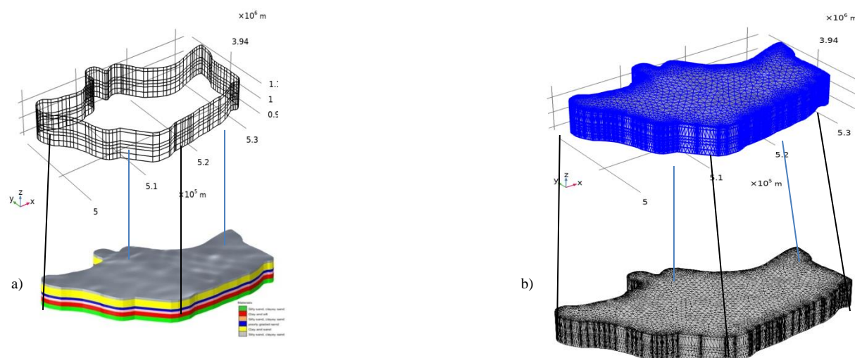
Fig. 6. a) Geological and topographic model and b) Three-dimensional discretization model
