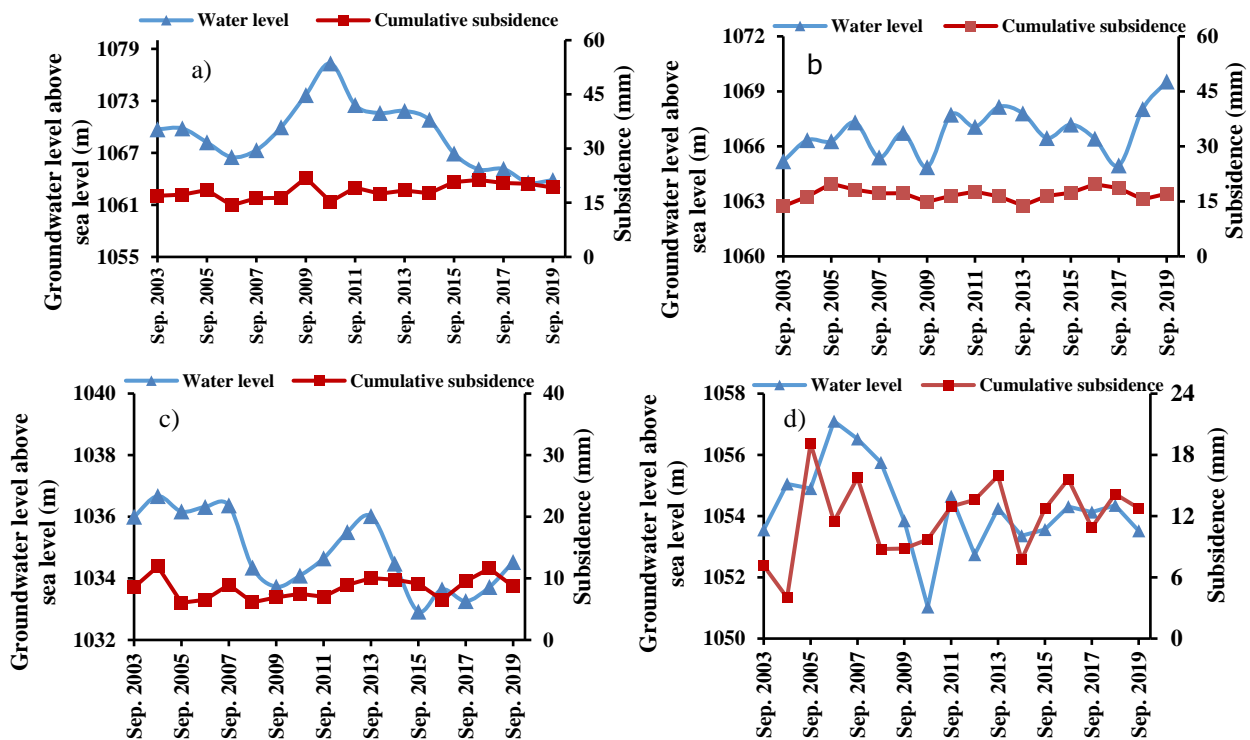
Fig. 13. Diagrams of the relationship subsidence with changes in aquifer levels in points a) Balaban,
