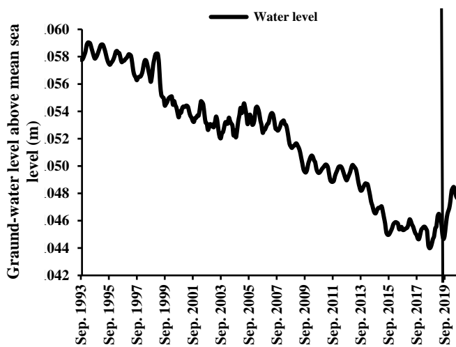
Fig. 3. Unit hydrograph of groundwater in Tehran-Shahriar plain, 1993-2019
