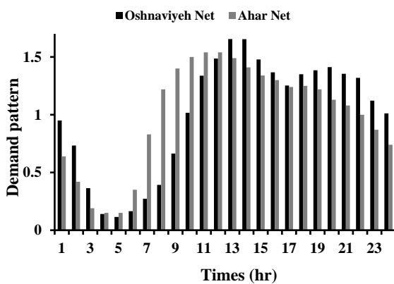
Fig. 3. Nodal Demand pattern in Ahar and Oshnaviyeh water distribution network
