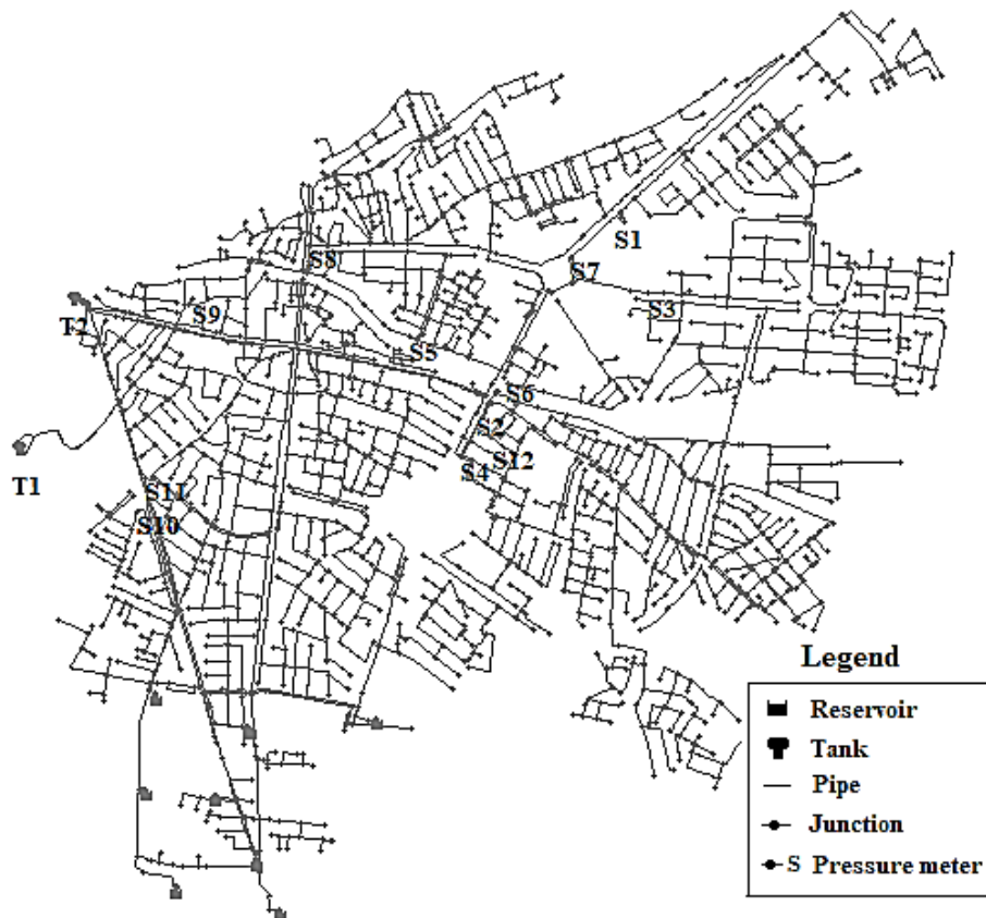
Fig. 2. Schematic of the Oshnaviyeh water distribution network
