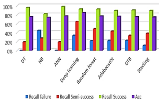
Fig. 4. Results of models accuracy with feature selection and LOF outlier data deletion
