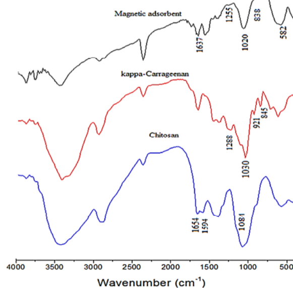
Fig. 2. FTIR spectra of chitosan, kappa-carrageenan, and magnetic adsorbent
