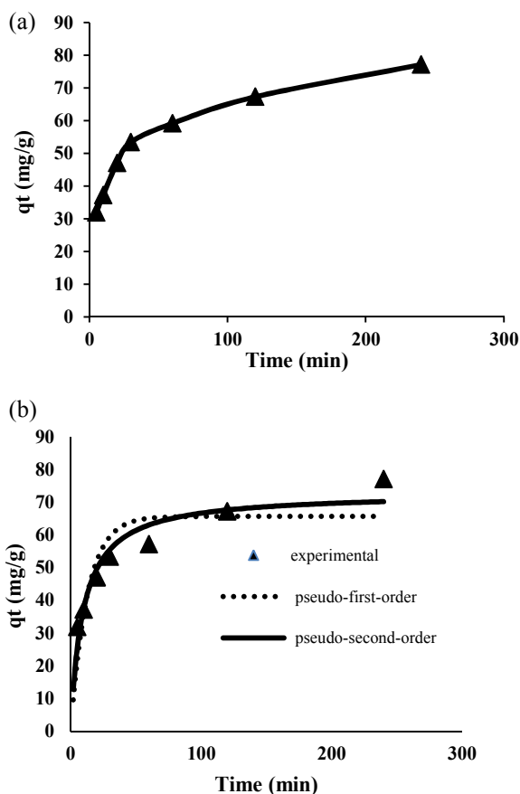
Fig. 9. (a) Effect of contact time on adsorption of EBT on magnetic nanocomposite (b) Non-linear fitting curves adsorption process according to pseudo-first-order and pseudo-second-order kinetic models
