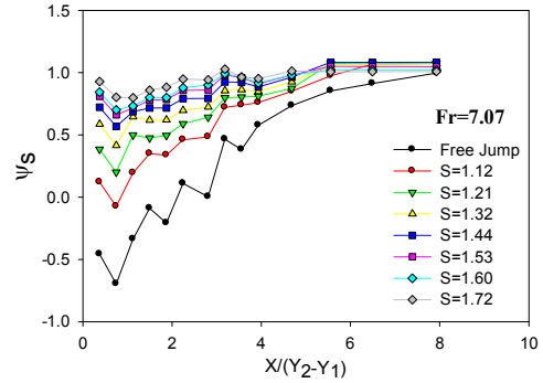
Fig. 11. Average variation of instant pressure in basin
