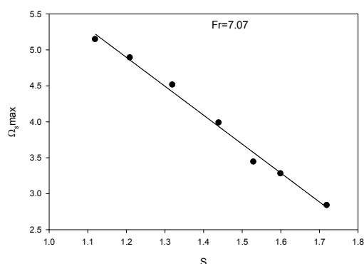
Fig. 15. Variation of coefficient \Omega_{Smax} related to submergence ratio
