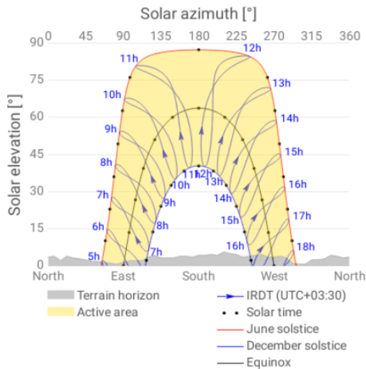
Fig. 4. The annual sun path in the study position to install photovoltaic power plant equipment
