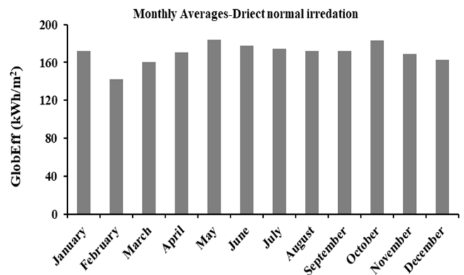
Fig. 6. Monthly average direct normal irradiation in location of canals
