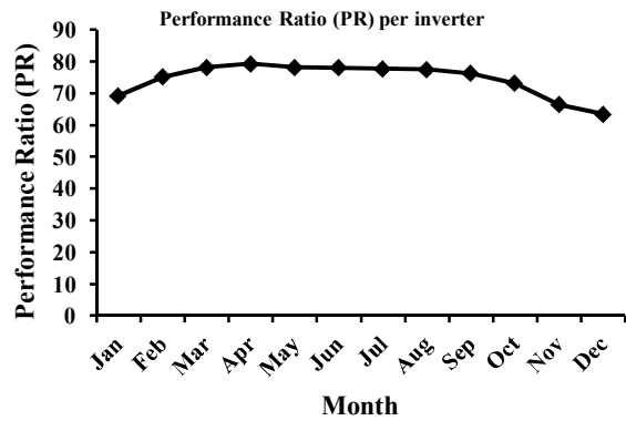
Fig. 9. Monthly performance ratio in Minab
