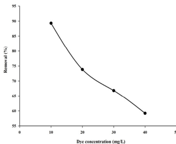
Fig. 7. Effect of initial concentration on malachite green adsorption onto GO/Fe 3 O 4 -Si-Pr-SH nanoparticles (adsorbent dosage: 0.01 g/L, equilibrium time: 60 min and pH=7)
