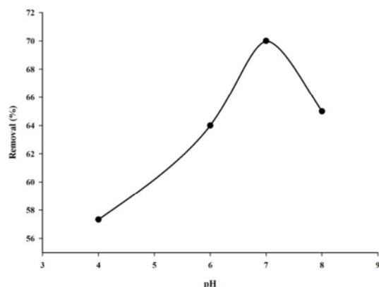
Fig. 6. Effect of pH on malachite green adsorption onto GO/Fe 3 O 4 -Si-Pr-SH nanoparticles (malachite green initial concentration: 10 mg/L, adsorbent dosage: 0.05 g/L, equilibrium time: 60 min)
