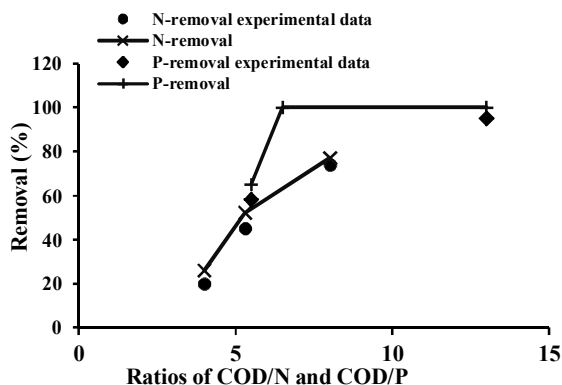
Fig. 6. Comparison of nitrogen and phosphorus removal by model and experiments at different COD/N and COD/P ratios
