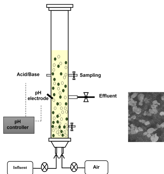
Fig. 1. Schematic representation of the reactor and the formed granules
