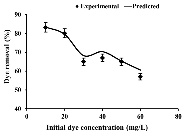
Fig. 12. Comparison between ANN predicted and experimental values of dye removal (%) as a function of initial dye concentration. Adsorption time = 20 min, adsorbent weight=0.5 g and \text{pH}=6.5
