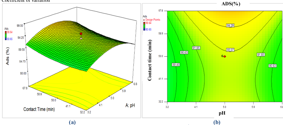
Fig. 8. (a) Surface, (b) contour plot for pH–contact time ( \text{Th}^{4+} concentration=55 mg/L)
