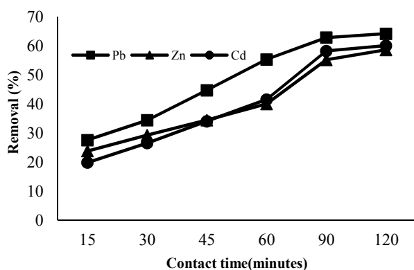
Fig. 7. Removal efficiency of heavy metals with respect to change in contact time
