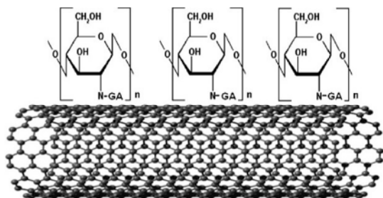
Fig.1. Structure of MWCNTs/CS
