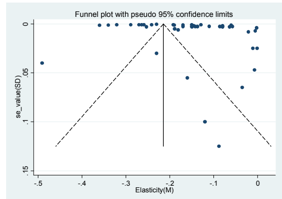
Fig. 1. The funnel plot for price elasticity vs. standard errors
