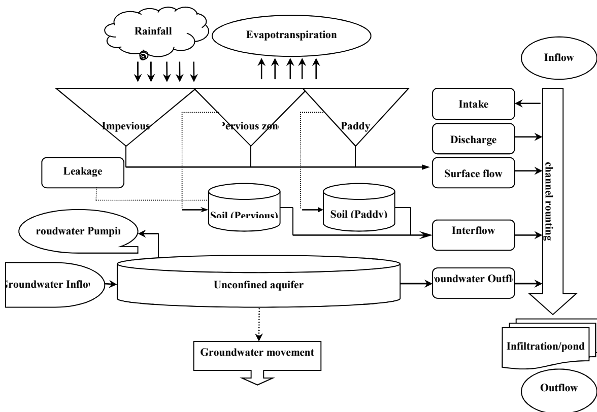
Fig. 1. Schematic diagram of hydrological cycle evaluation (Miller et al. 2014)
