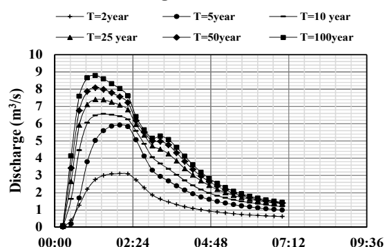
Fig. 8. Output hydrograph of the watershed after its development with penetration measures effected
