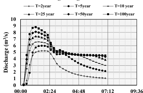
Fig. 7. Output hydrograph of the watershed after its development with storage measures effected
