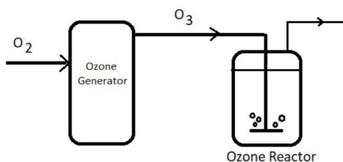
Fig. 1. Schematic of waste water ozonation
