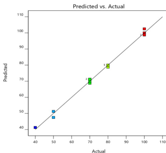
Fig. 4. Predicted response value of E. coli removal efficiency vs. actual value
