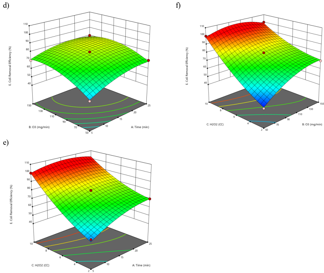
Fig. 2. 3D response surface diagram for COD and E. coli reduction as a function of a) ozonation duration and ozone amount (amount of H 2 O 2 at central value), b) amount of H 2 O 2 and ozonation duration (amount of ozone in the central value), c) amount of ozone and amount of H 2 O 2 (ozonation duration in the central value), d) ozonation duration and ozone amount (amount of H 2 O 2 at central value), e) amount of H 2 O 2 and ozonation duration (amount of ozone in the central value), f) amount of ozone and amount of H 2 O 2 (ozonation duration in the central value)
