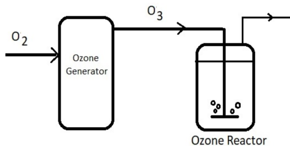
Fig. 1. Schematic of waste water ozonation
