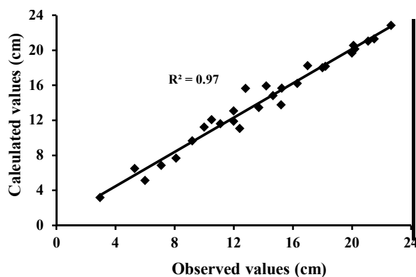
Fig. 7. Fitting diagram of observed values based on calculated subsidence values
