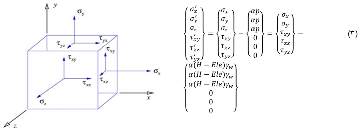
Fig. 5. Stress components in the three-dimensional model
