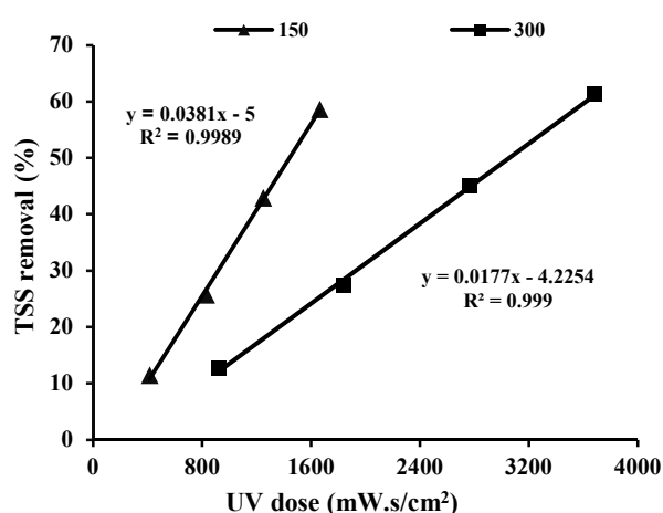
Fig. 4. TSS removal efficiency versus UV dose
