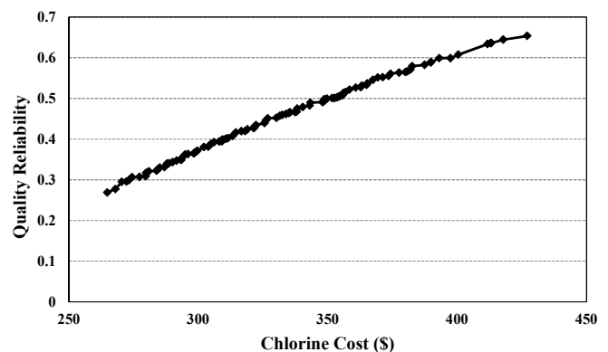
Fig. 8. Pareto curve of the second approach based on the DDSM method
