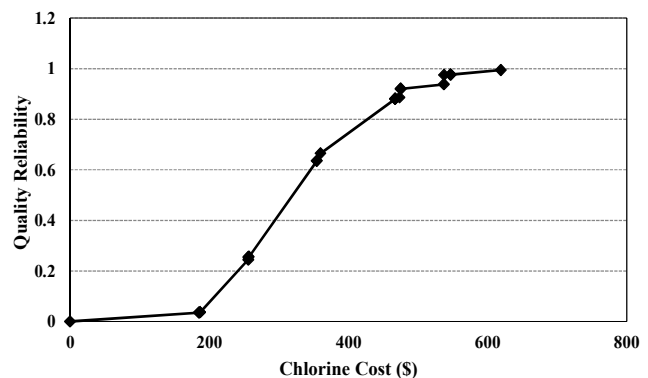
Fig. 5. Pareto curve of the first approach for a constant injection rate but a variable pump rotation
