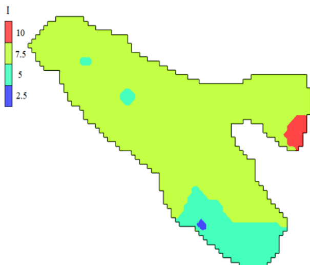
Fig. 7. Rating of parameter I (impact of the existing status of seawater intrusion) in the GALDIT model for Qom aquifer
