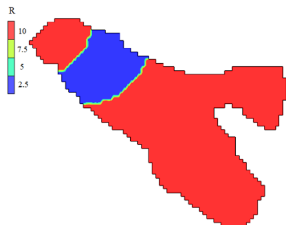
Fig. 9. Rating of parameter R (aquifer recharge) in the GALDITR model for Qom aquifer
