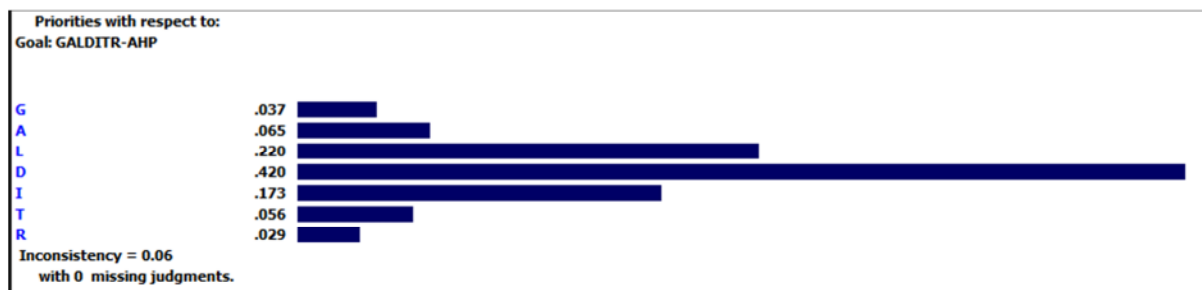
Fig. 12. Histogram of weight of GALDITR indicators using AHP method in Qom aquifer
