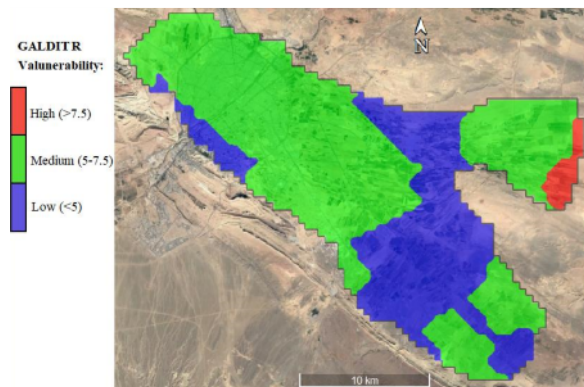
Fig. 11. Vulnerability map of Qom aquifer using GALDIT model
