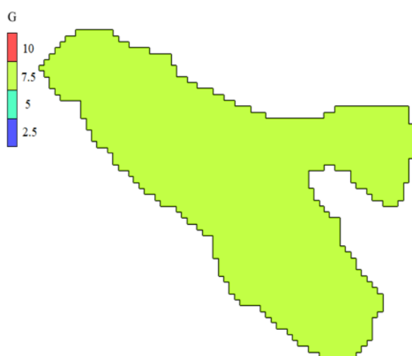
Fig. 2. Rating of parameter G (aquifer type) in the GALDIT model for Qom aquifer
