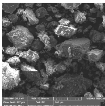
Fig. 2. Scanning electron microscopy images of powder particles travertine stone with scale 2 and 100 μ
