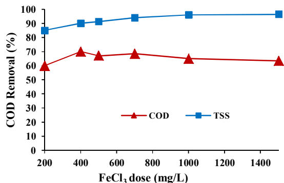
Fig. 2. Ferric chloride optimum dose for coagulation process
