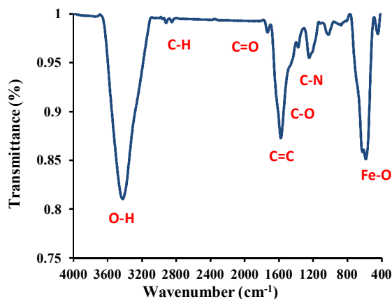
Fig. 3. FTIR spectra of MGO-IDA
