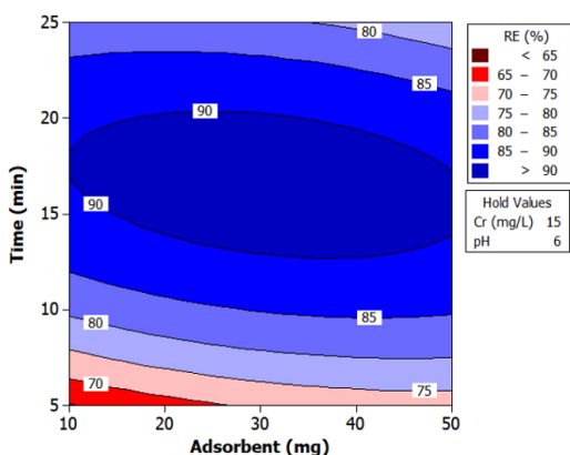
Fig. 4. Two and three-dimensional diagrams of the effect of adsorption time and adsorbent weight on adsorption efficiency
