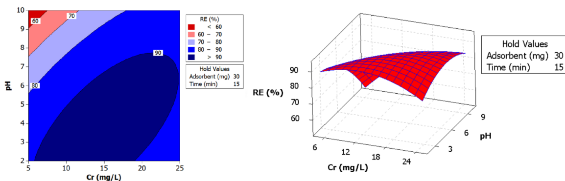
Fig. 7. Two and three-dimensional diagrams of the effect of pH and \text{Cr}^{3+} concentration on adsorption efficiency
