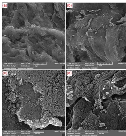
Fig. 1. SEM images of a) GO, b) MGO, c) MGO-IDA before Cr ion adsorption and d) MGO-IDA after Cr ion adsorption
