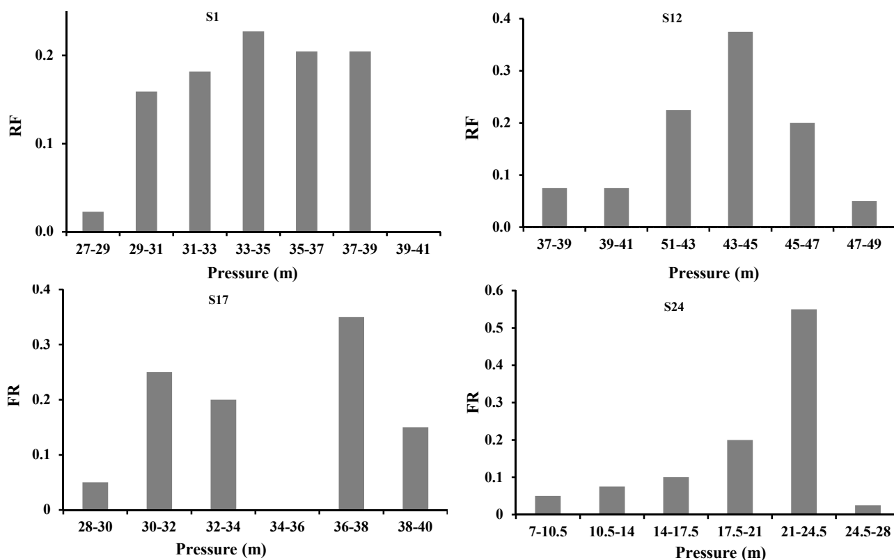
Fig. 6. Frequency variation of nodal pressure data for the maximum consumption time at different stations of the water distribution network of Ahar
