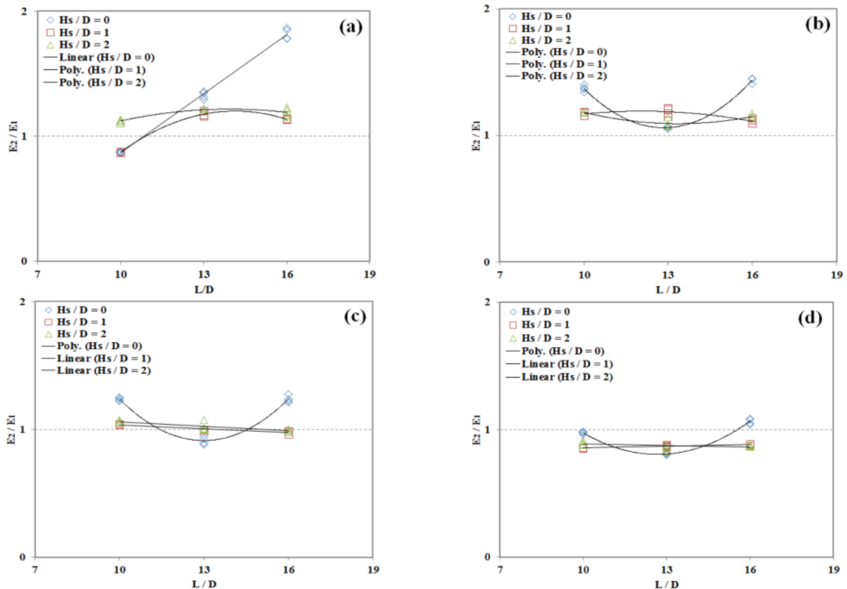
Fig. 7. Variations of E_2/E_1 versus L/D values for various F_r numbers: a) F_r=1.77 ; b) F_r=2.01 ; c) F_r=2.18 and d) F_r=2.32
