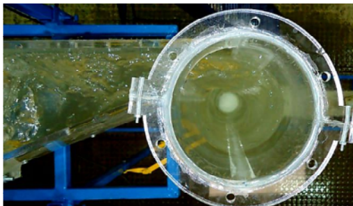
Fig. 5. The vortex flow observed at the beginning of the vertical shaft
