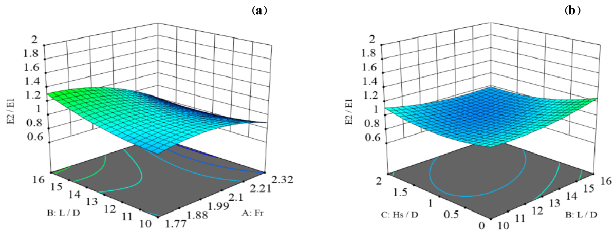
Fig. 12. Response surface plots: a) Effect of F_r and L/D on the E_2/E_1 ; b) Effect of L/D and H_s/D on the E_2/E_1
