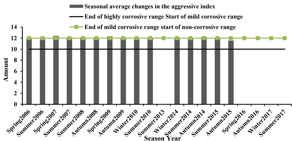
Fig. 7. Average aggressive index of water supply resources of Dehdasht and Sough city during the 2006-2017 seasons
